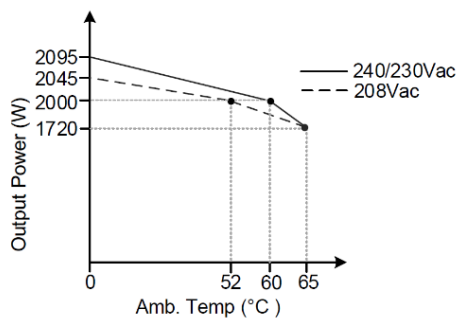
Fig. 1 Q2000 AC Output Power vs Temperature Profile.
