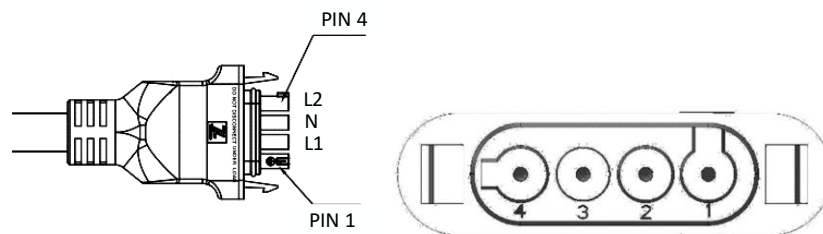
Figure 24: Pin configuration for AC cables
