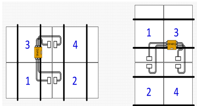
Figure 3: Q2000 – Rectangle arrangement (landscape [left] and portrait [right]).
