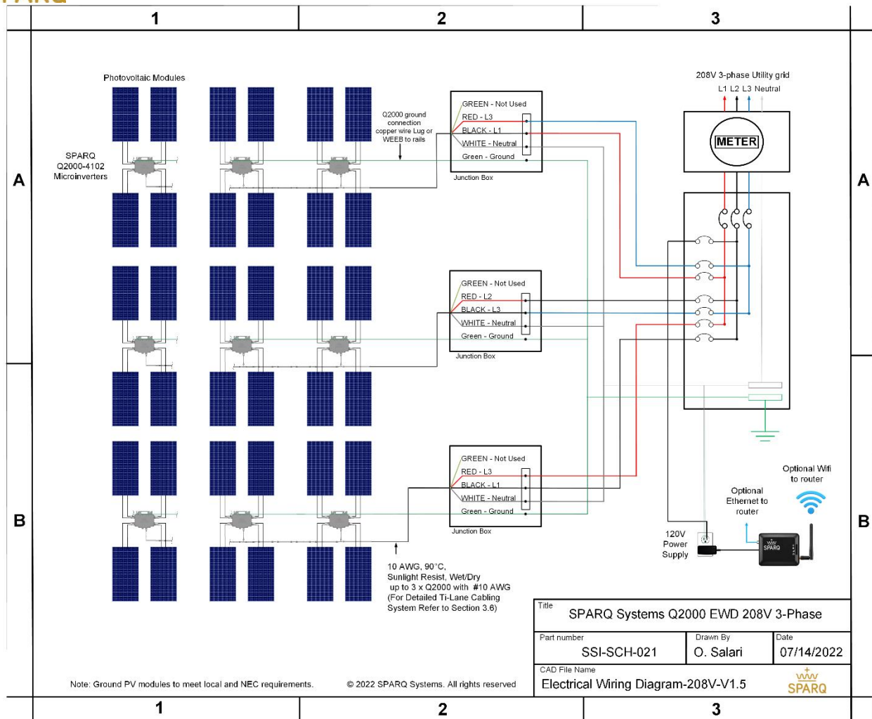
Figure 29: Single line diagram for three phase system.
