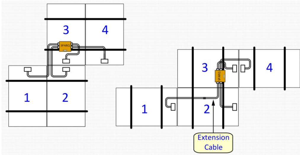
Figure 7: Q2000 - S-shaped arrangements.
