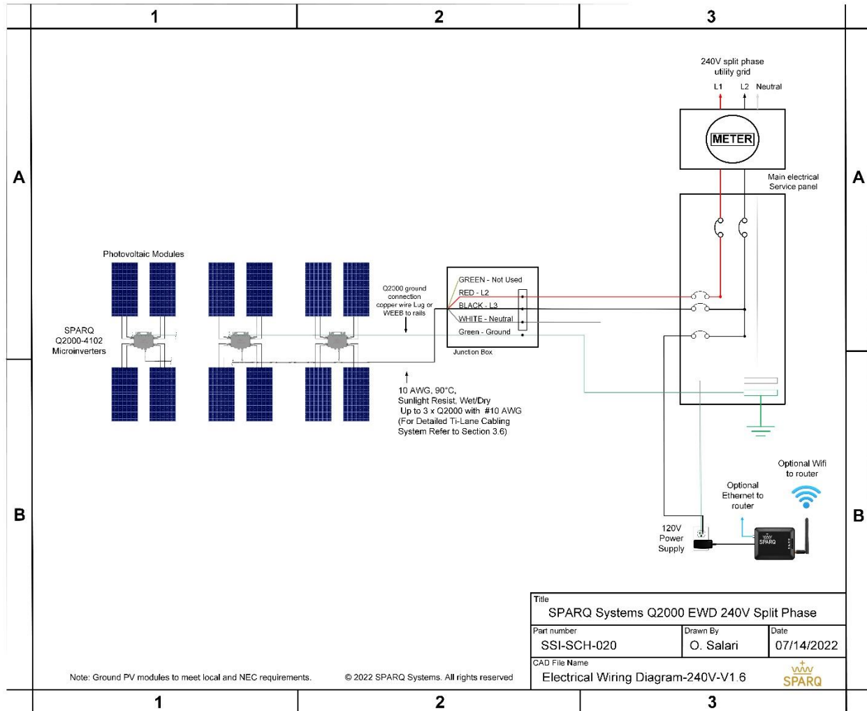
Figure 28: Single line diagram for single phase system.
