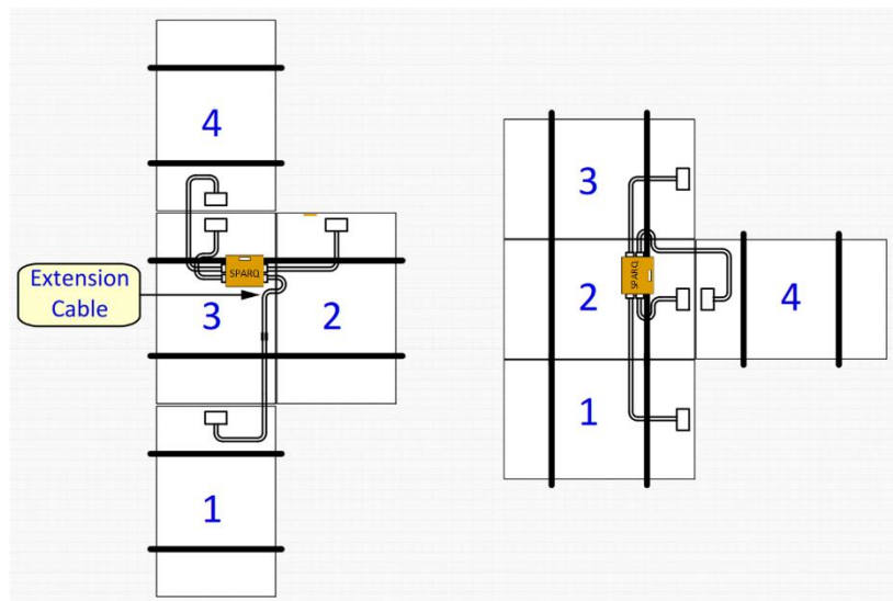
Figure 6: Q2000 T-shape arrangements.
