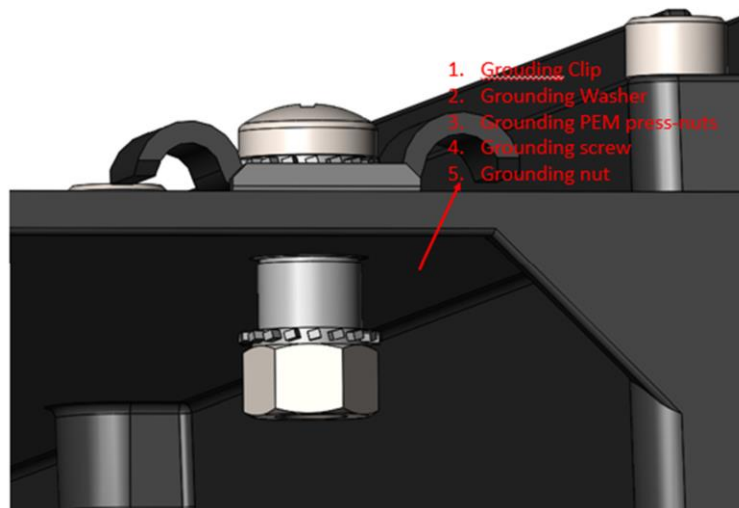
Figure 26: Grounding the micro inverter.
