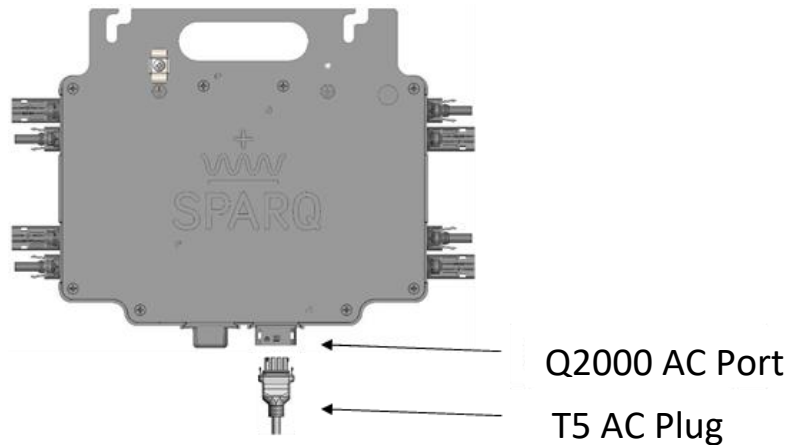
Figure 19: SPARQ microinverter connection with T5 AC plug.
