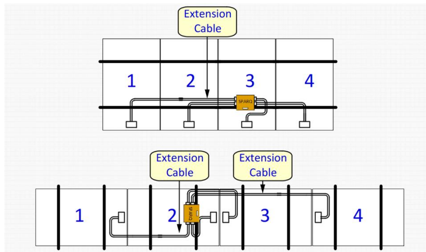
Figure 4: Q2000 – Row of four arrangement.
